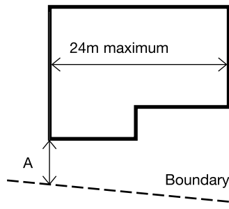
Diagram 22 Permitted unprotected areas for Method 1
