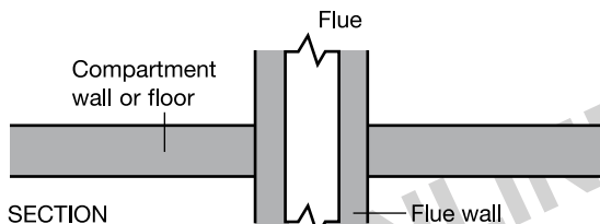
a. FLUE PASSING THROUGH COMPARTMENT WALL OR FLOOR
